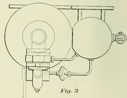
A REINFORCED BRAKE.
